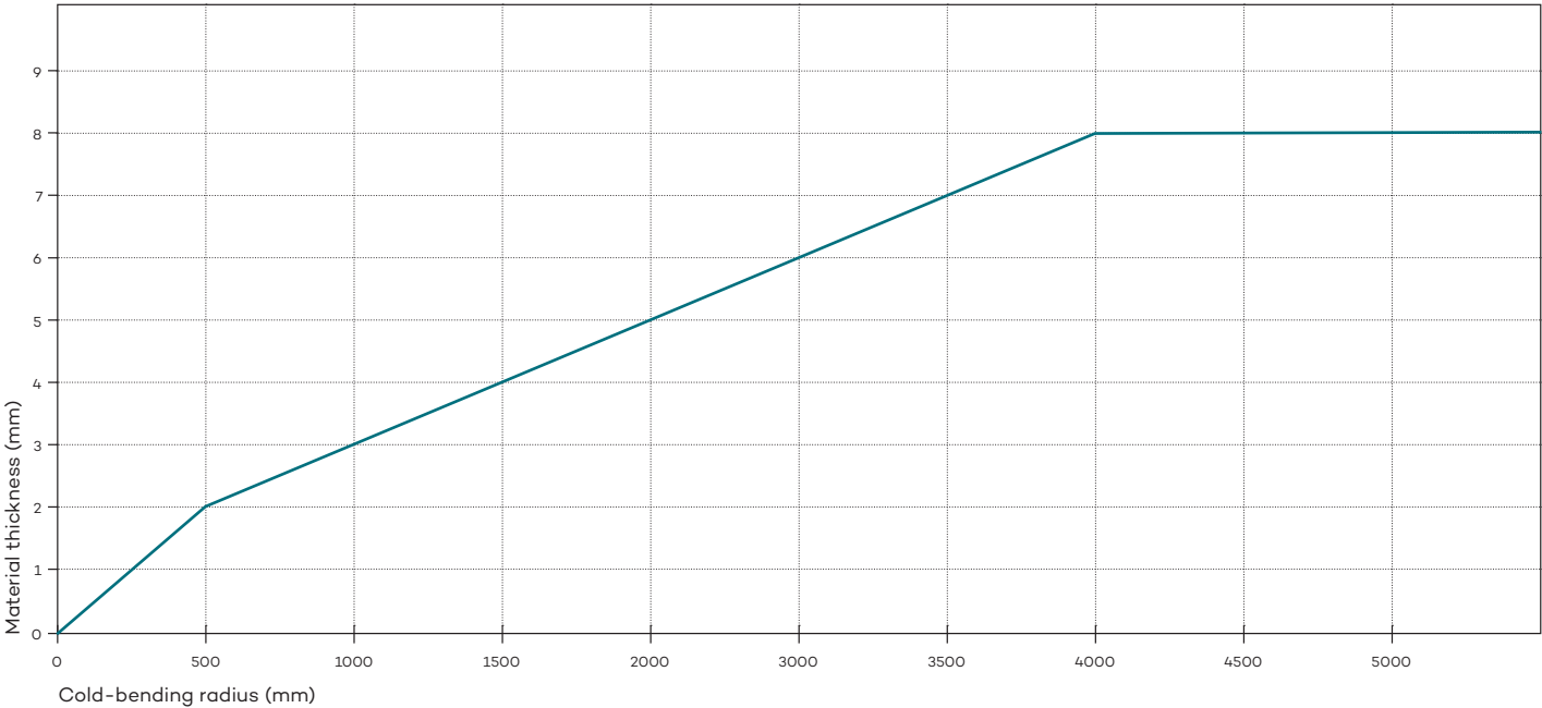
Sheet thickness in mm for barrel vaults with a hoop spacing of 1,000 mm and a wind pressure/snow load (radial pressure) of 750 N/m²
